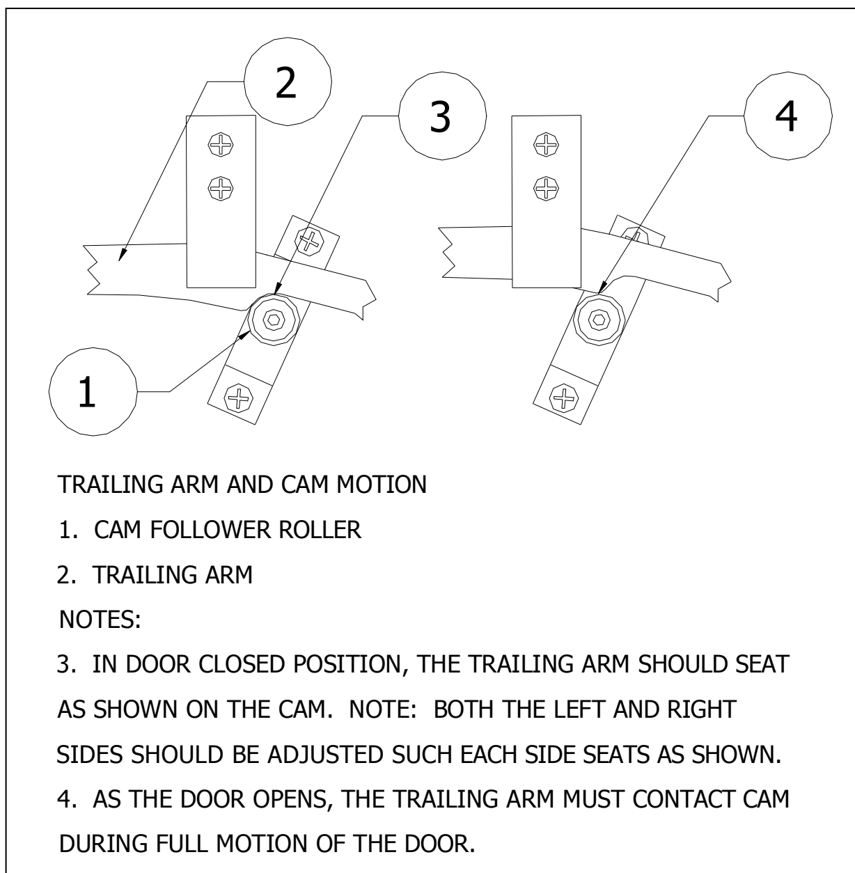
Figure 7-4 Trailing Arm and Cam Motion
